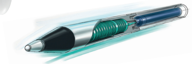
Patronen-Roller-System/uma cartridge roller system
